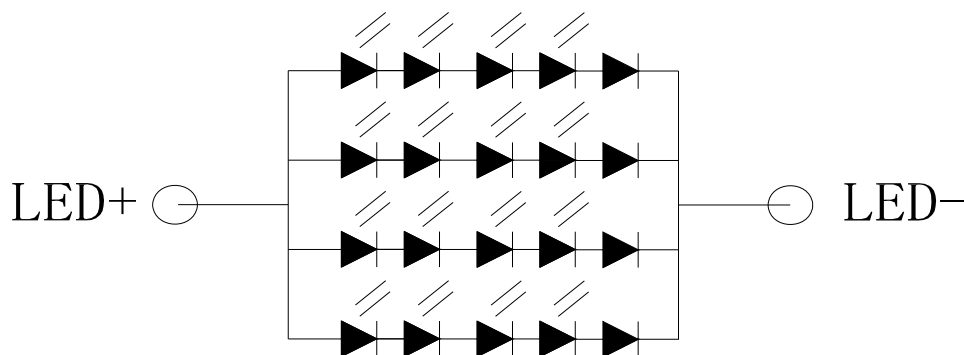
B/L Circuit
